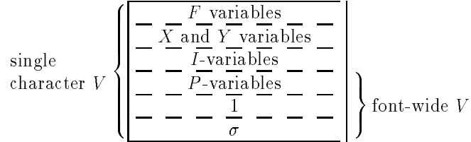
Figure 37: The structure of the vector V
