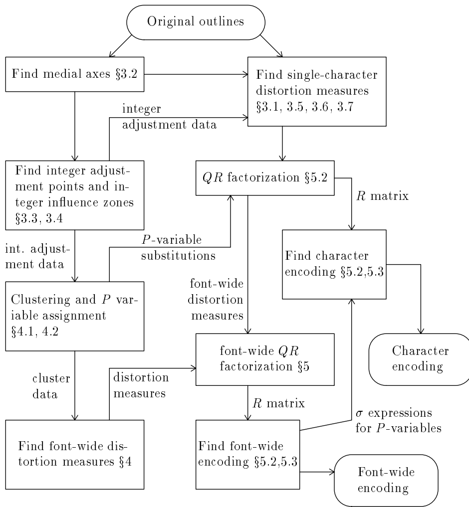
Figure 41: The flow of intermediate results when going from outlines to the encoded forms.
