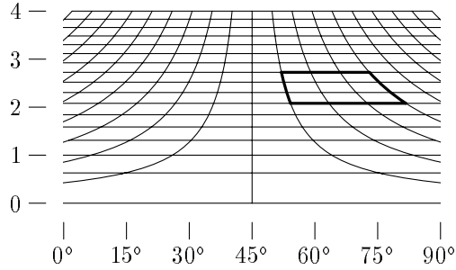
Figure 33: Square buckets of size \frac{1}{3} in (u, v) space mapped into (\theta, w) space by using \gamma_1 = \gamma_2 = 1 and \theta_0 = 45^\circ in (22). Potential width clusters for integer offset intervals are three-by-three blocks such as the one outlined in bold.
